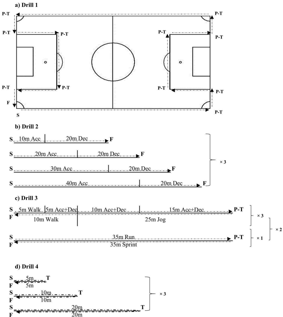
Figure 1. Layout and sequence for each drill. S – start, F – finish, P-T – pause-turn, Acc – acceleration, Dec – deceleration.
